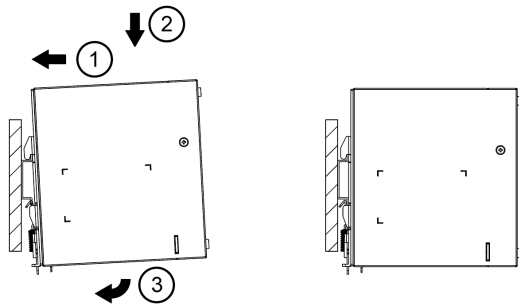
Fig. 3.1 Mounting
