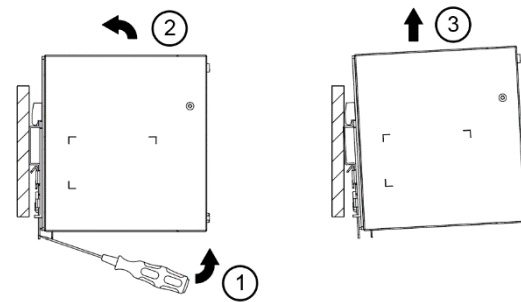
Fig. 3.2 Dismounting
