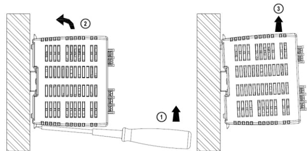
Fig. 2.2 Dismounting
