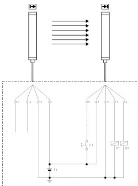
Wiring example
